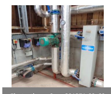
Electrotherm Spec 801271-60, 60 litre mild steel low loss heater
