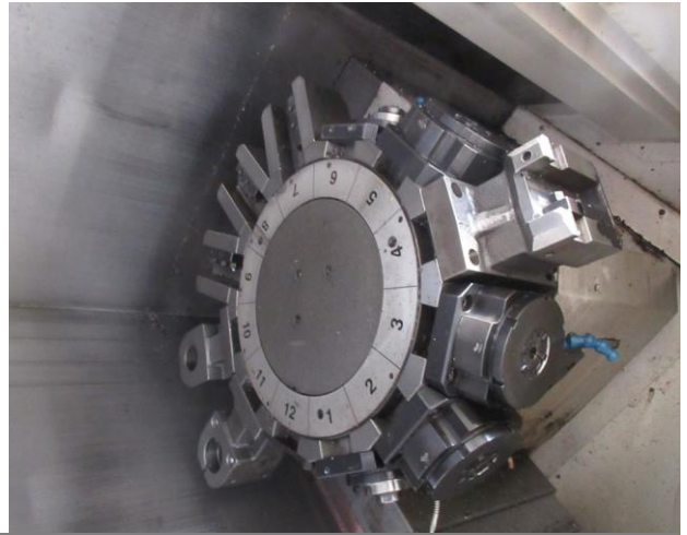
Mazak Quick Turn Smart 350M CNC slant bed turning centre (2015), Mazatrol Smart control, 12 station turret with live tooling
