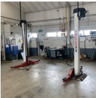
Stenhoj 2 post vehicle lift 5000kg type 004703 Maestro DK-7150 barrit (2004)
